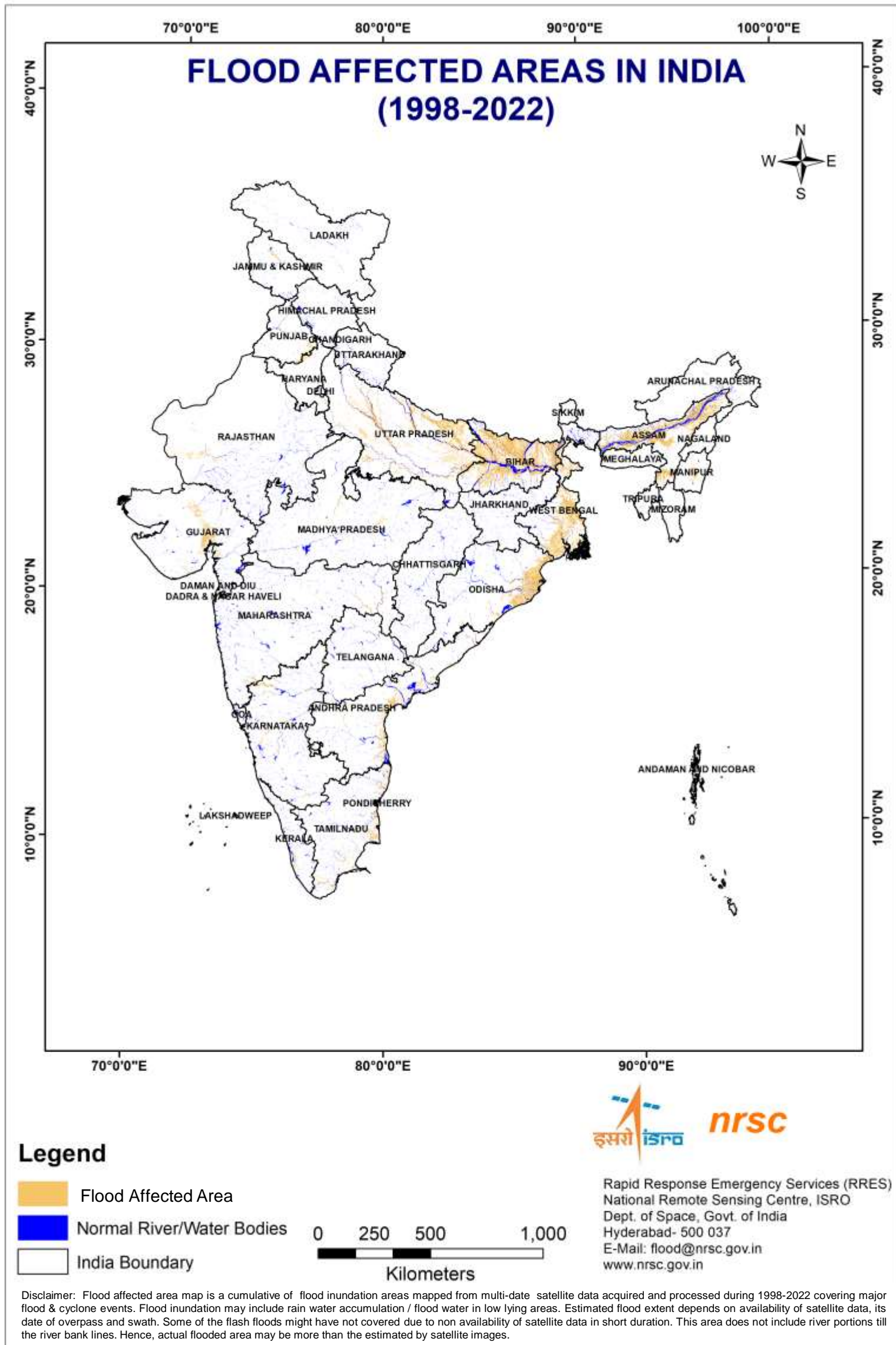
Figure.5.1. Flood Affected Area in India
