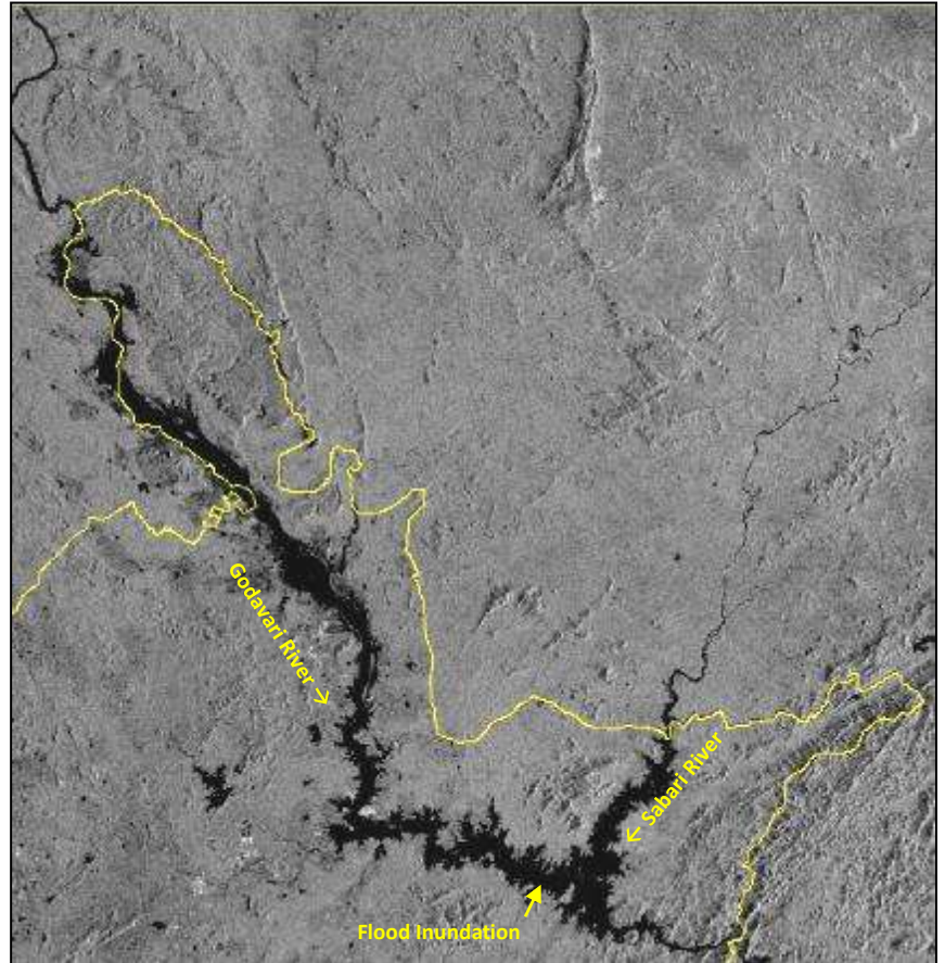
Radarsat image of 07-Aug-2006
