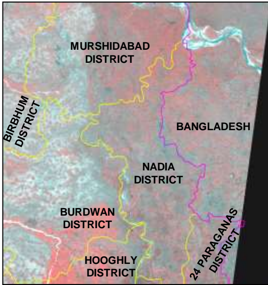
IRS 1C WiFS image of 10 Oct, 2000
