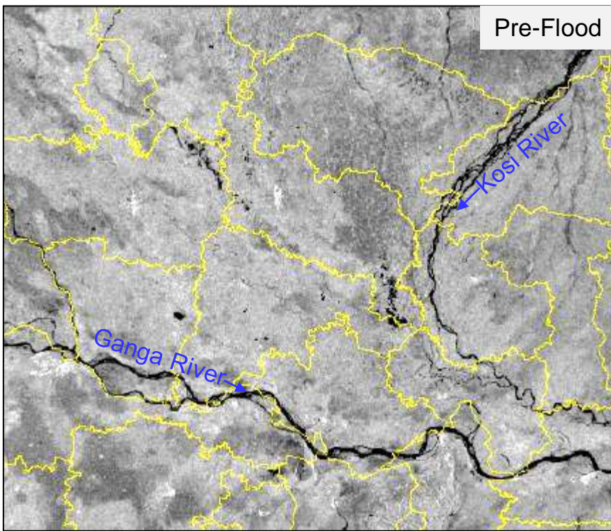
Radarsat image of 04-Jul-2007
