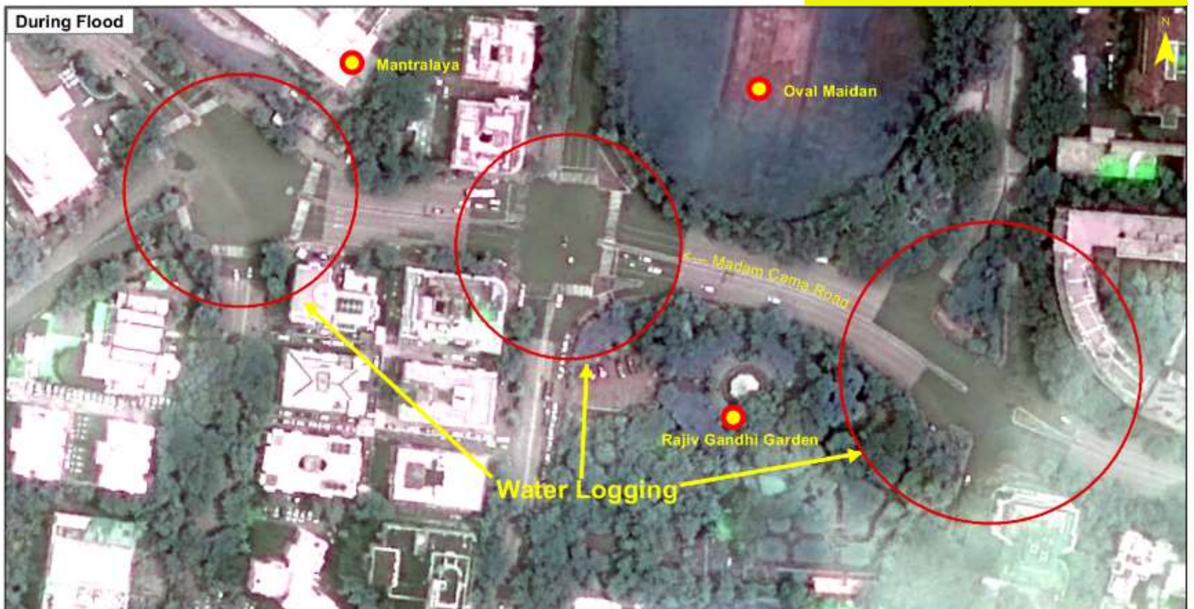
PLEIADES Image of 09 August 2020
