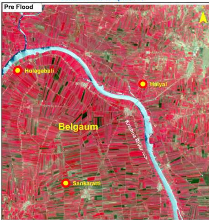
Sentinel-2A of 19-April-2021
