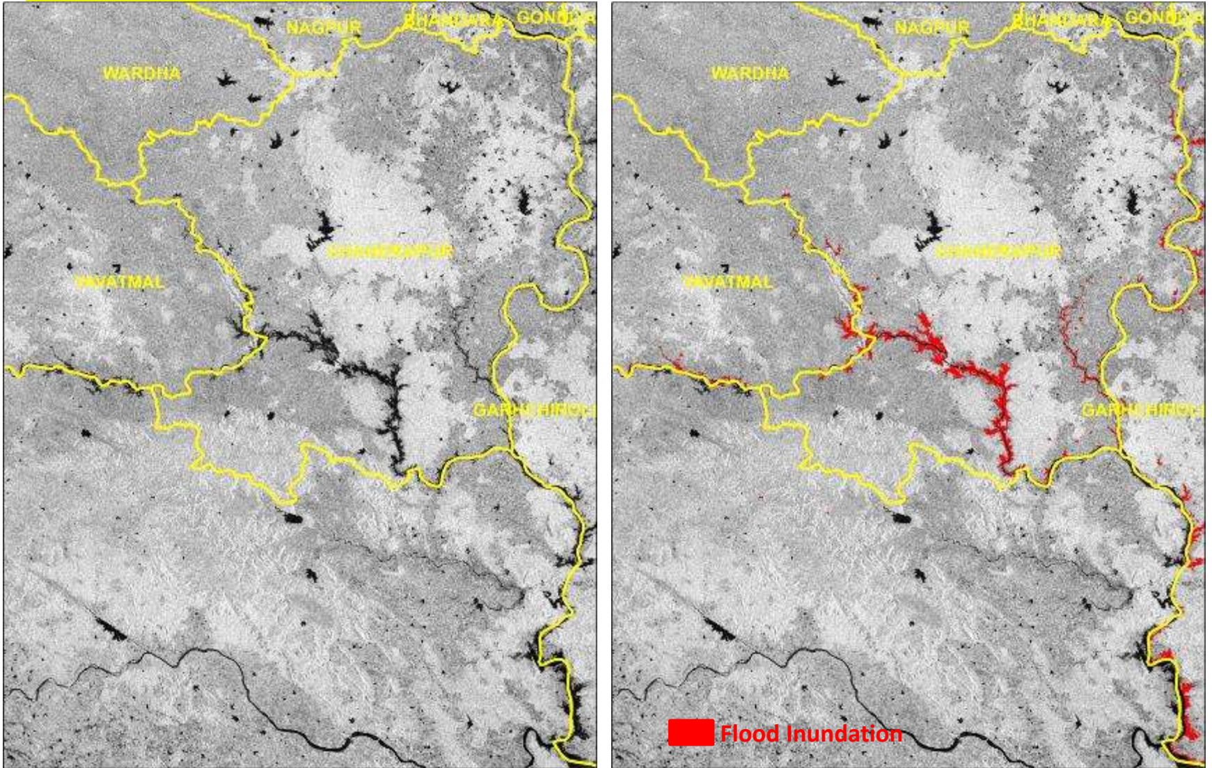
RADARSAT 2 Image of 1 st August 2013
