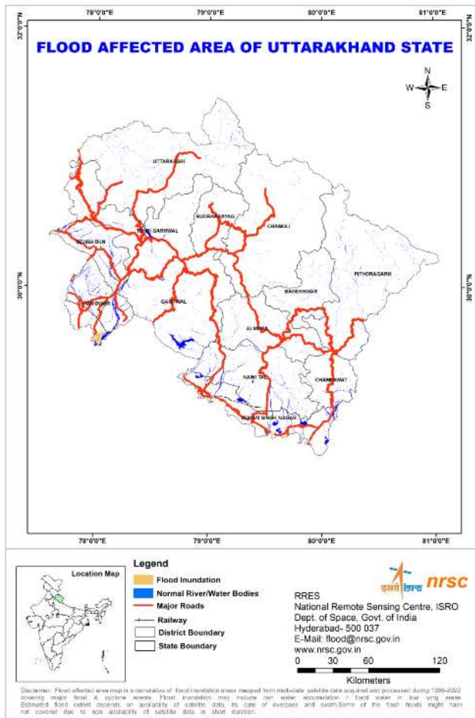
Fig.30.1 Flood affected area in Uttarakhand State
