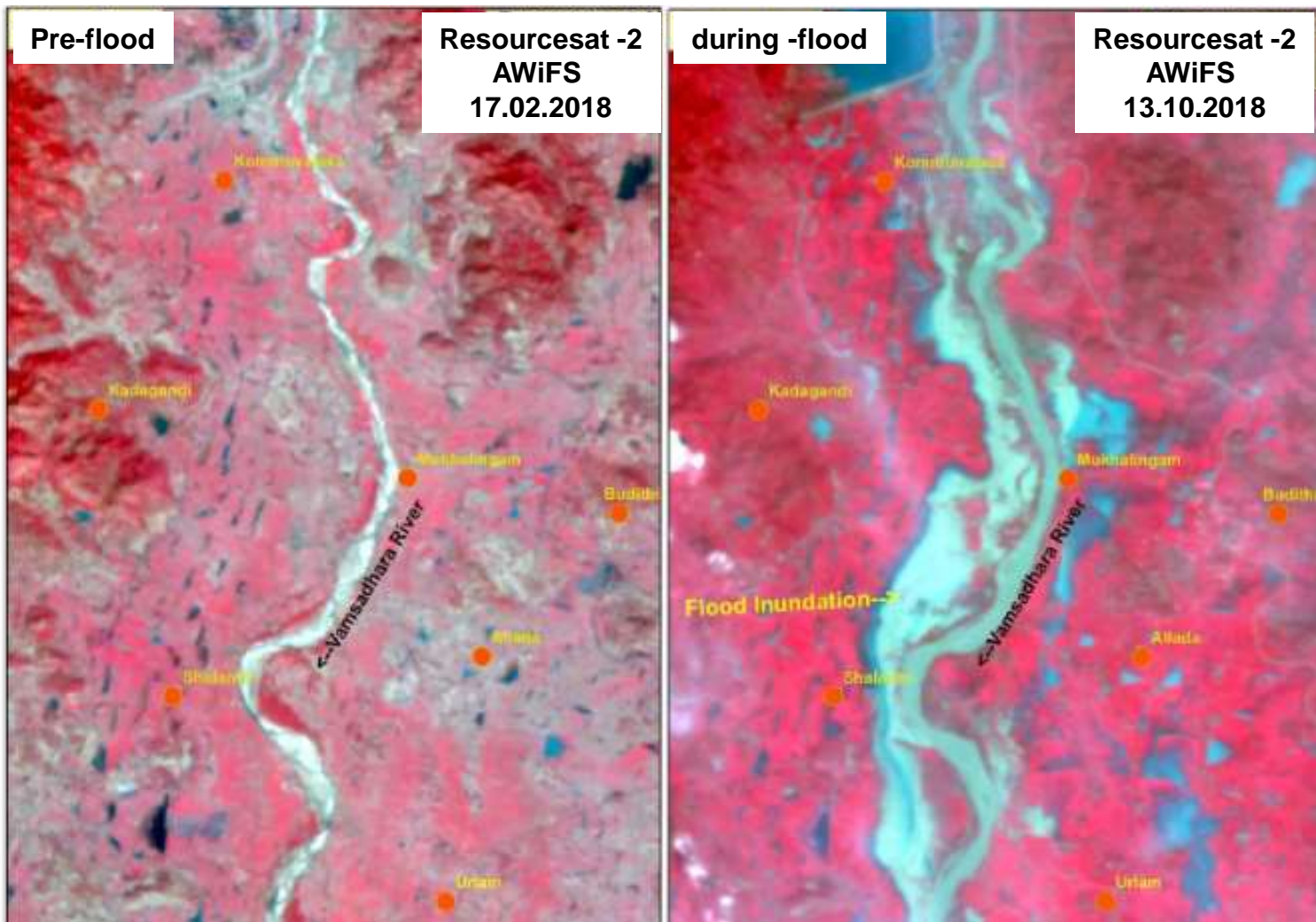
Flood affected areas in Srikakulam district during 2018 due to Cyclone Titli
