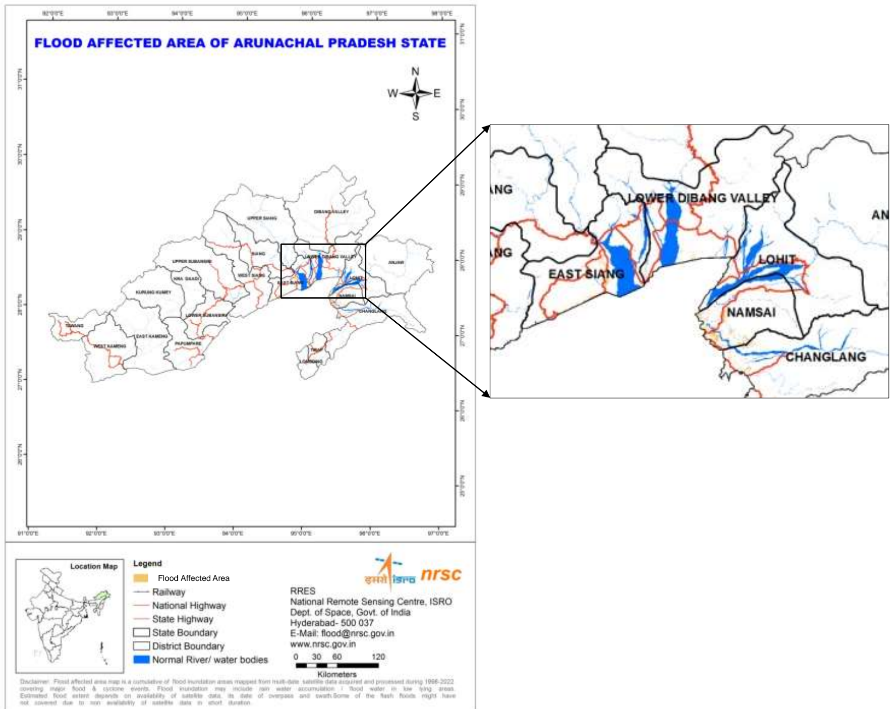
Fig.7.1 Flood affected area in Arunachal Pradesh
