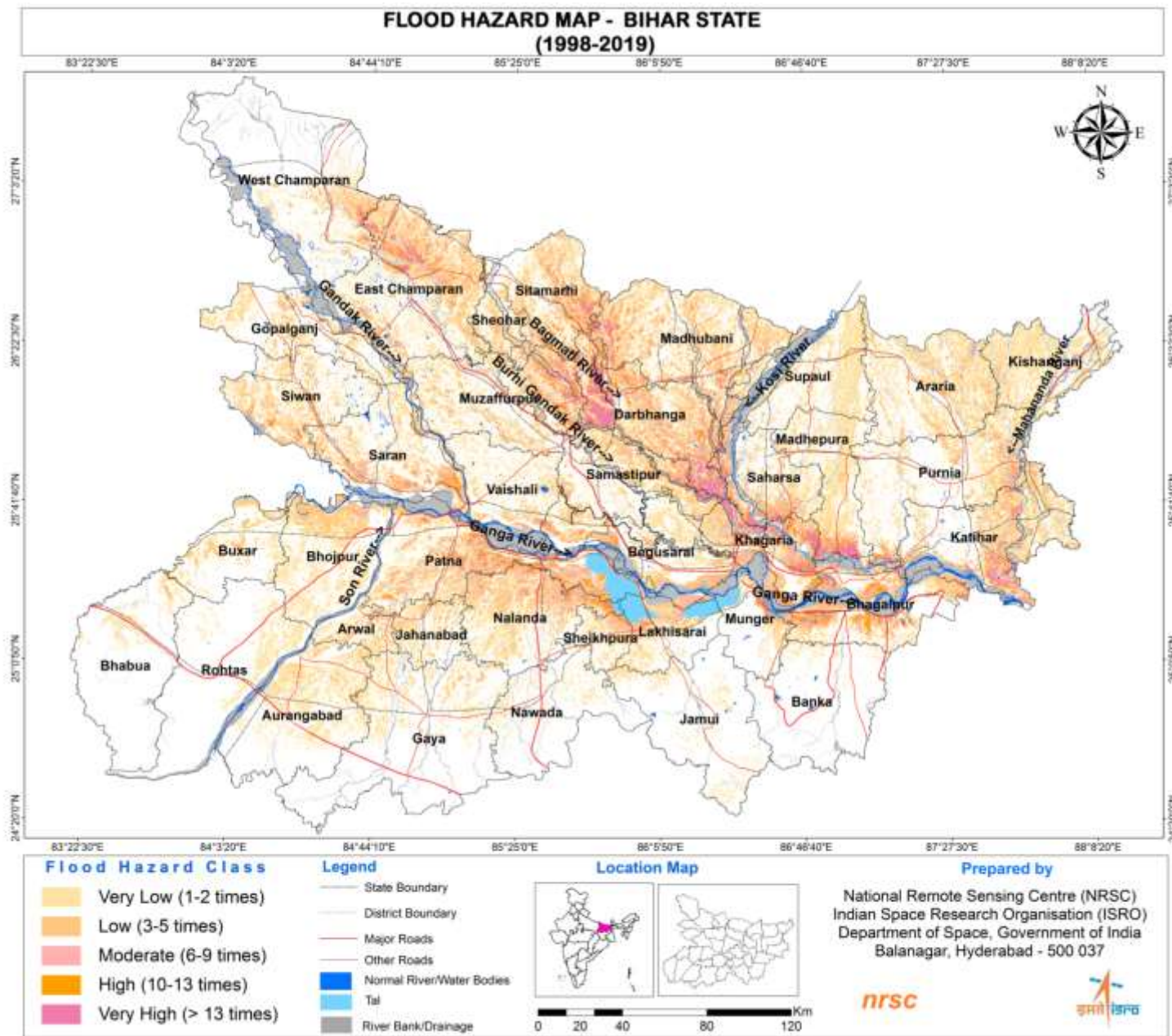
Fig.9.1 Flood Hazard map of Bihar
