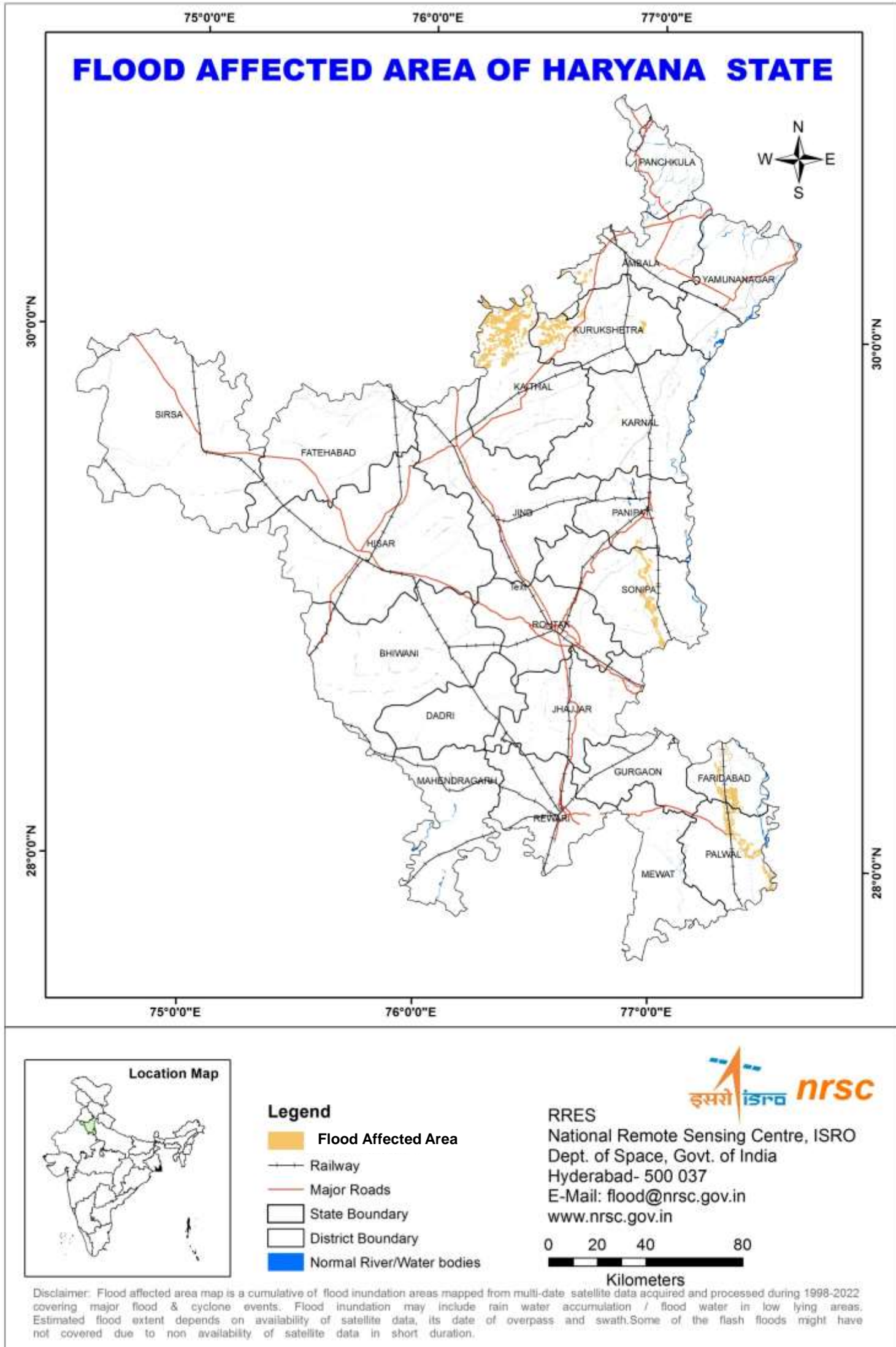
Fig.13.1 Flood affected area in Haryana State
