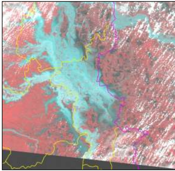
IRS 1C WiFS image of 10 Oct, 2000
