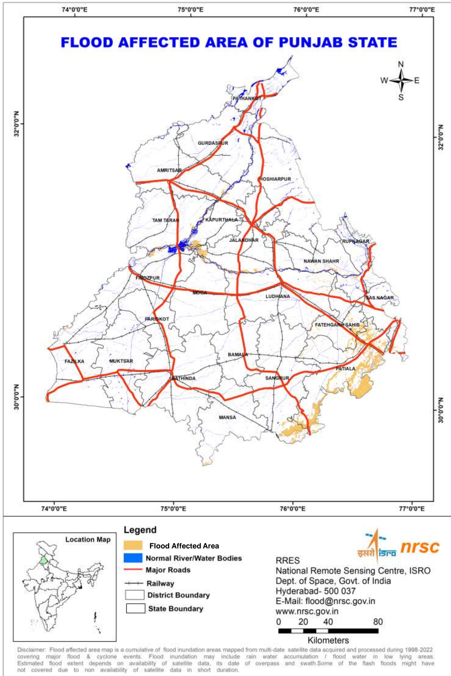
Fig.24.1 Flood affected area in Punjab State
