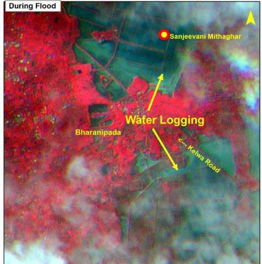
Resoucesat-2 L4FMX Image of 18-July-2021
