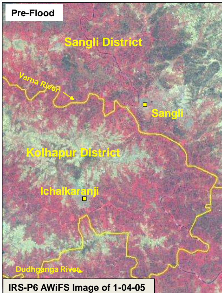
Satellite Images of part of Sangli & Kolhapur Districts Maharashtra State
