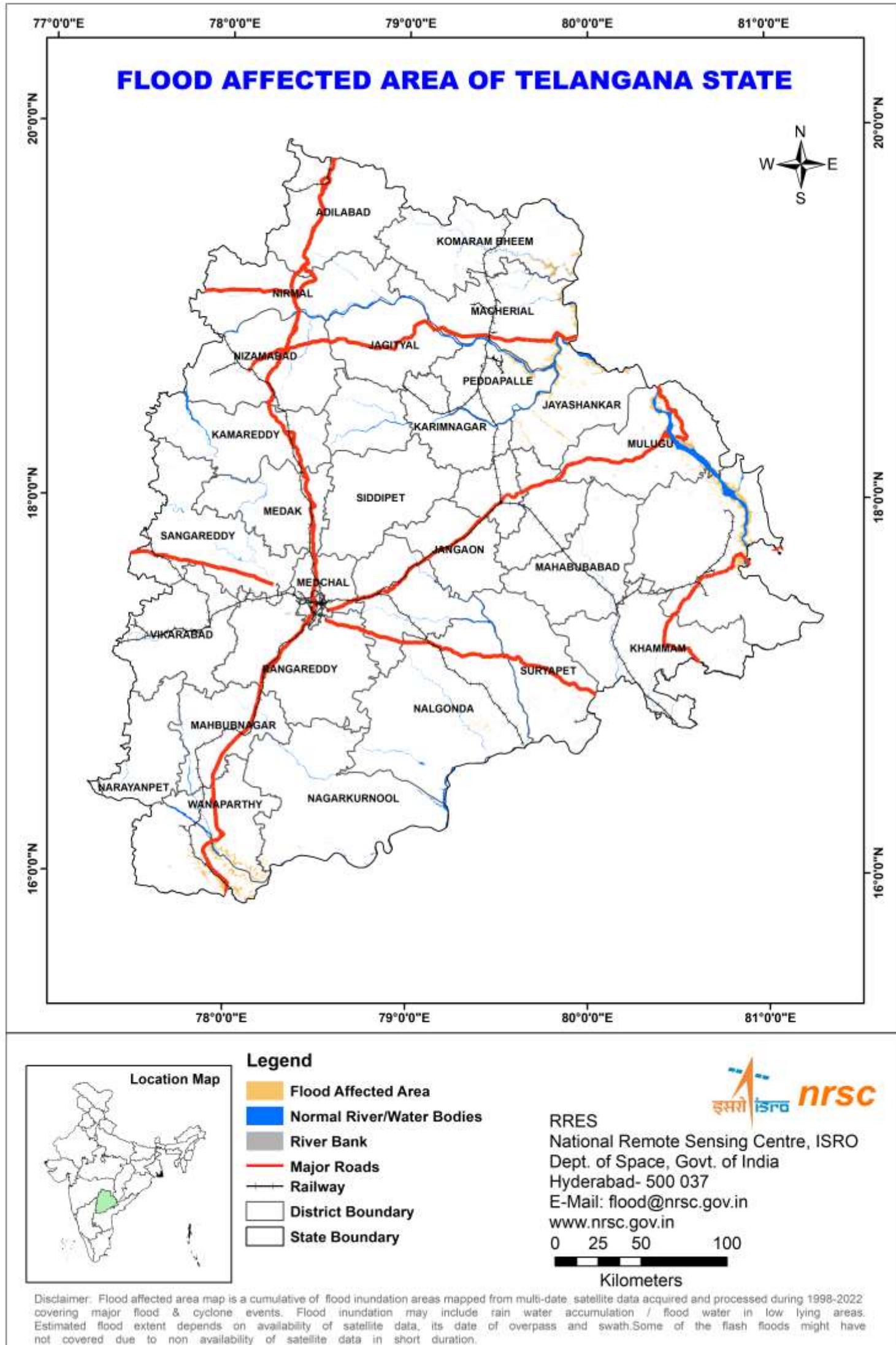
Fig.27.1 Flood affected area in Telangana State
