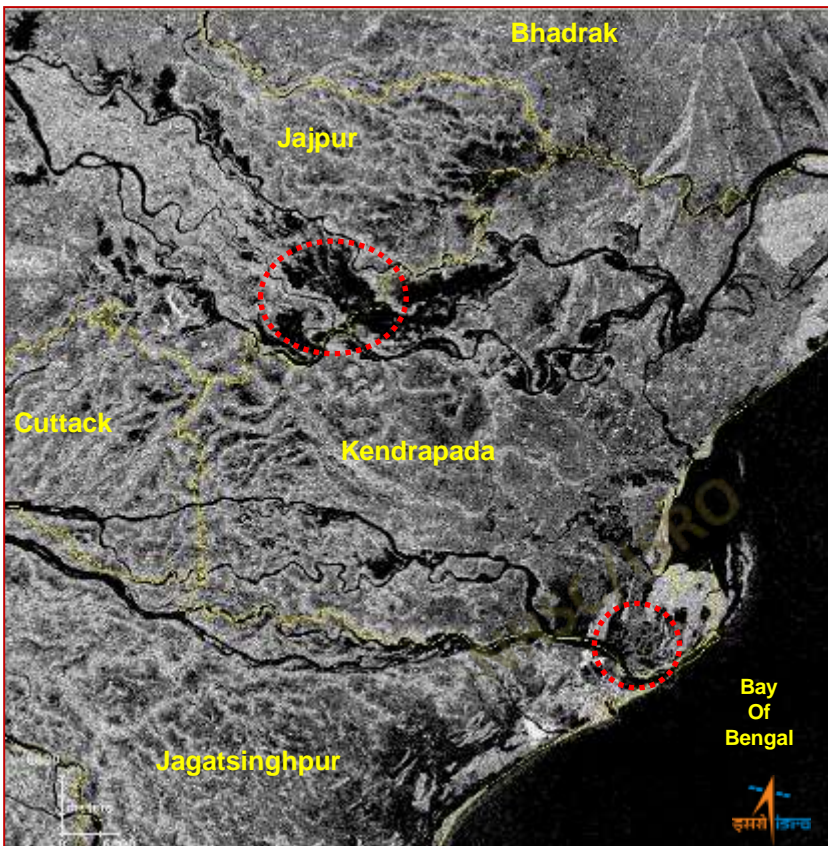
RADARSAT image of 12-Oct-2013 (17:48 hours IST)
