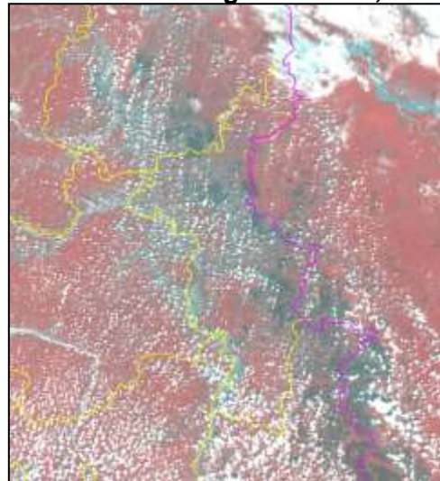
IRS 1D WiFS image of 20 Oct, 2000
