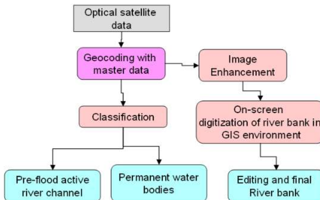
Figure.3.1. Flowchart for Pre-flood Data Preparation
