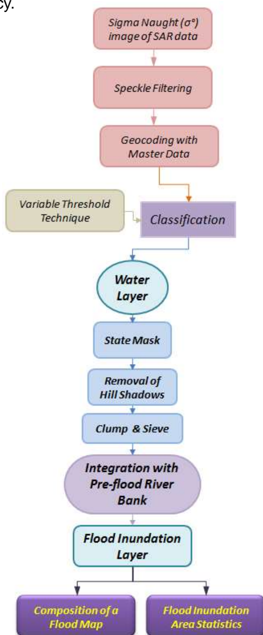
Fig.4.1 Methodology for flood mapping and monitoring by SAR satellite data
