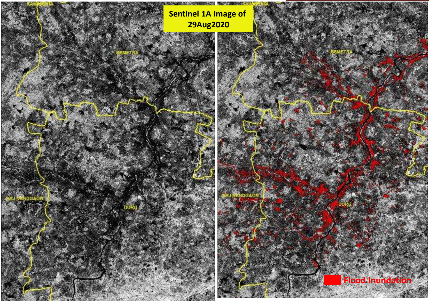
Sentinel 1A Image of 29th Aug2020
