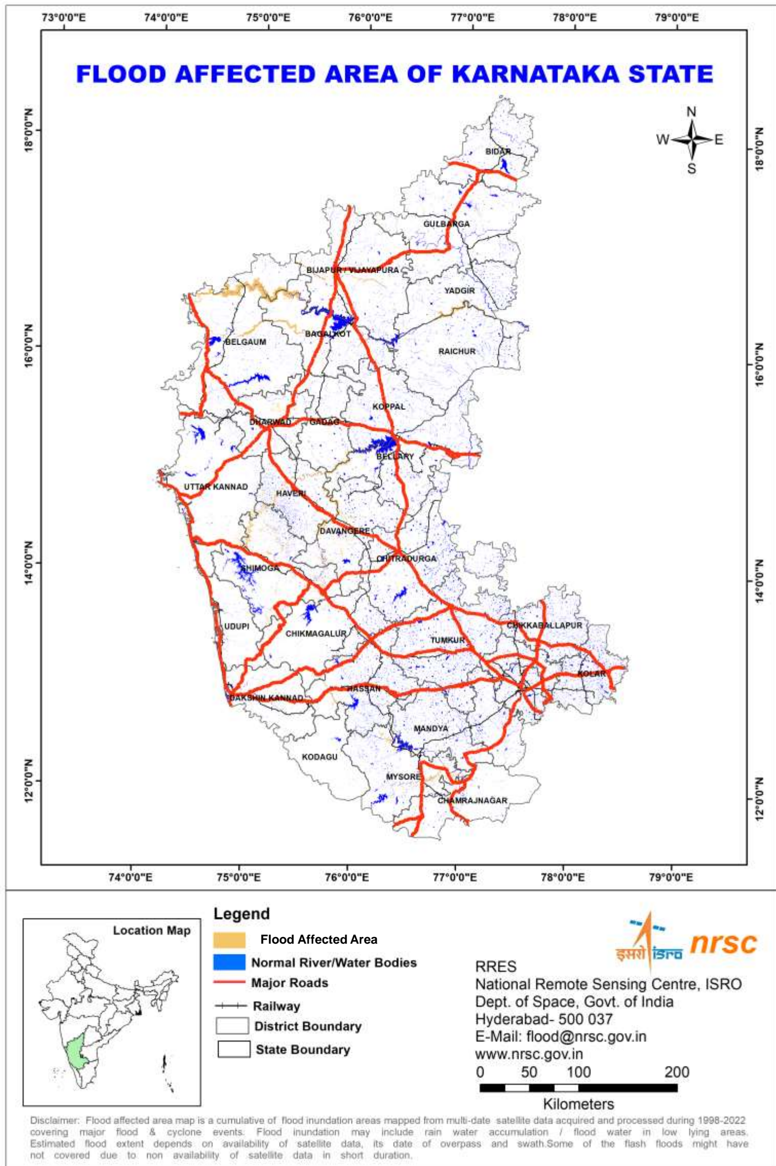
Fig.17.1 Flood affected area in Karnataka
