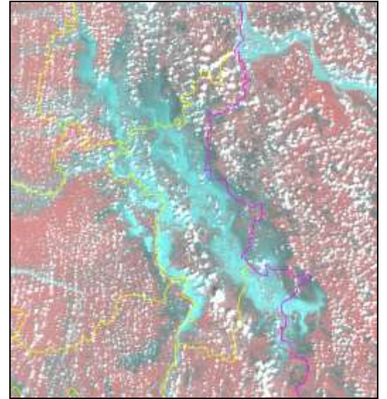
IRS 1D WiFS image of 20 Oct, 2000
