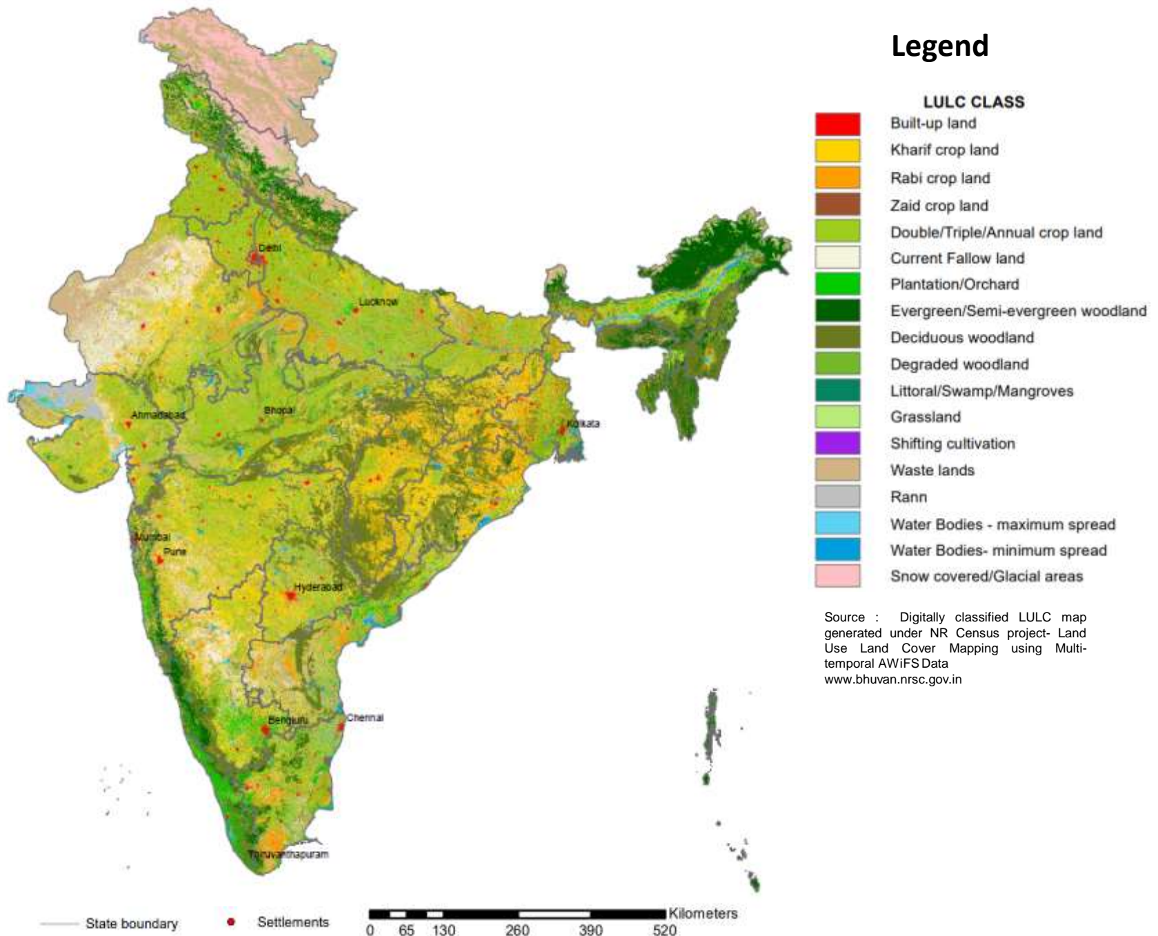
Figure.3.2. Satellite derived Landuse / Landcover Map (2021-22) at 1: 250,000 scale
