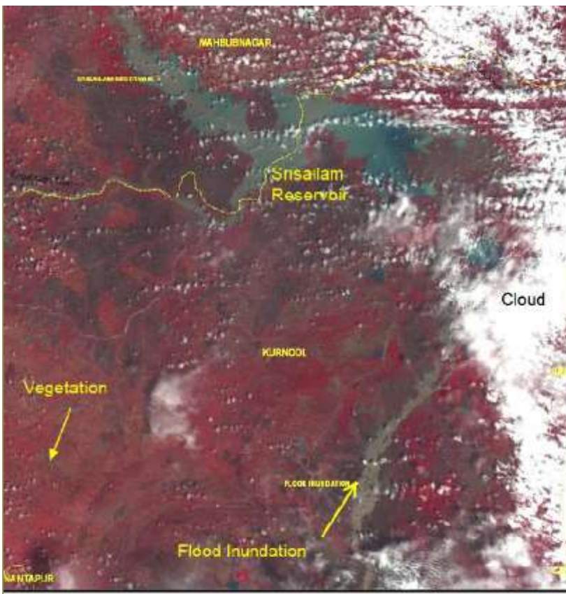
Resourcesat AWiFS as on 04 th Oct 2009
