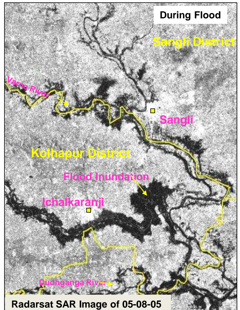
Satellite Images of part of Sangli & Kolhapur Districts Maharashtra State
