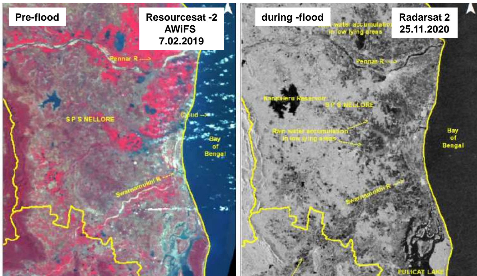
Flood affected areas in part of Nellore district, Andhra Pradesh during Cyclone -NIVAR
