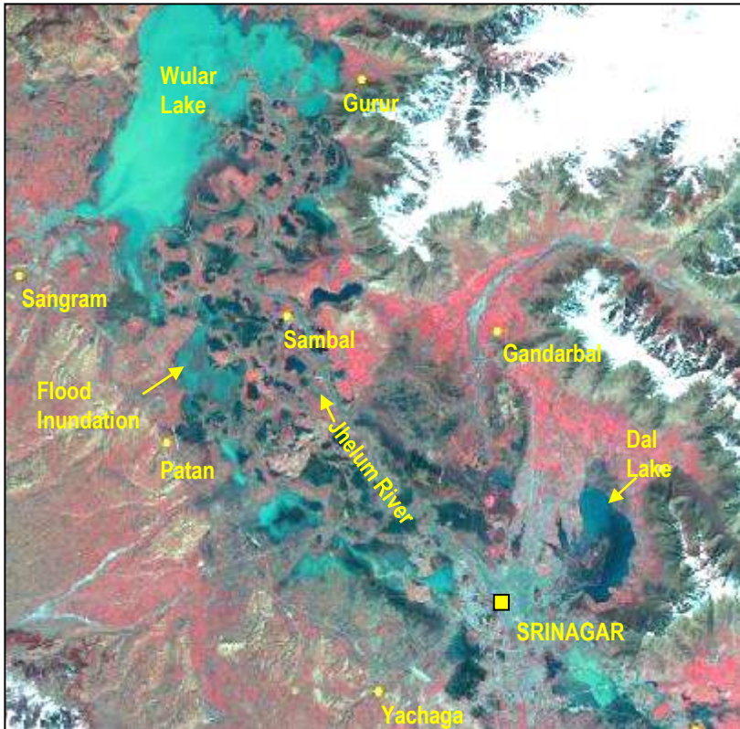
Flood situation as on 26-Mar-2007
