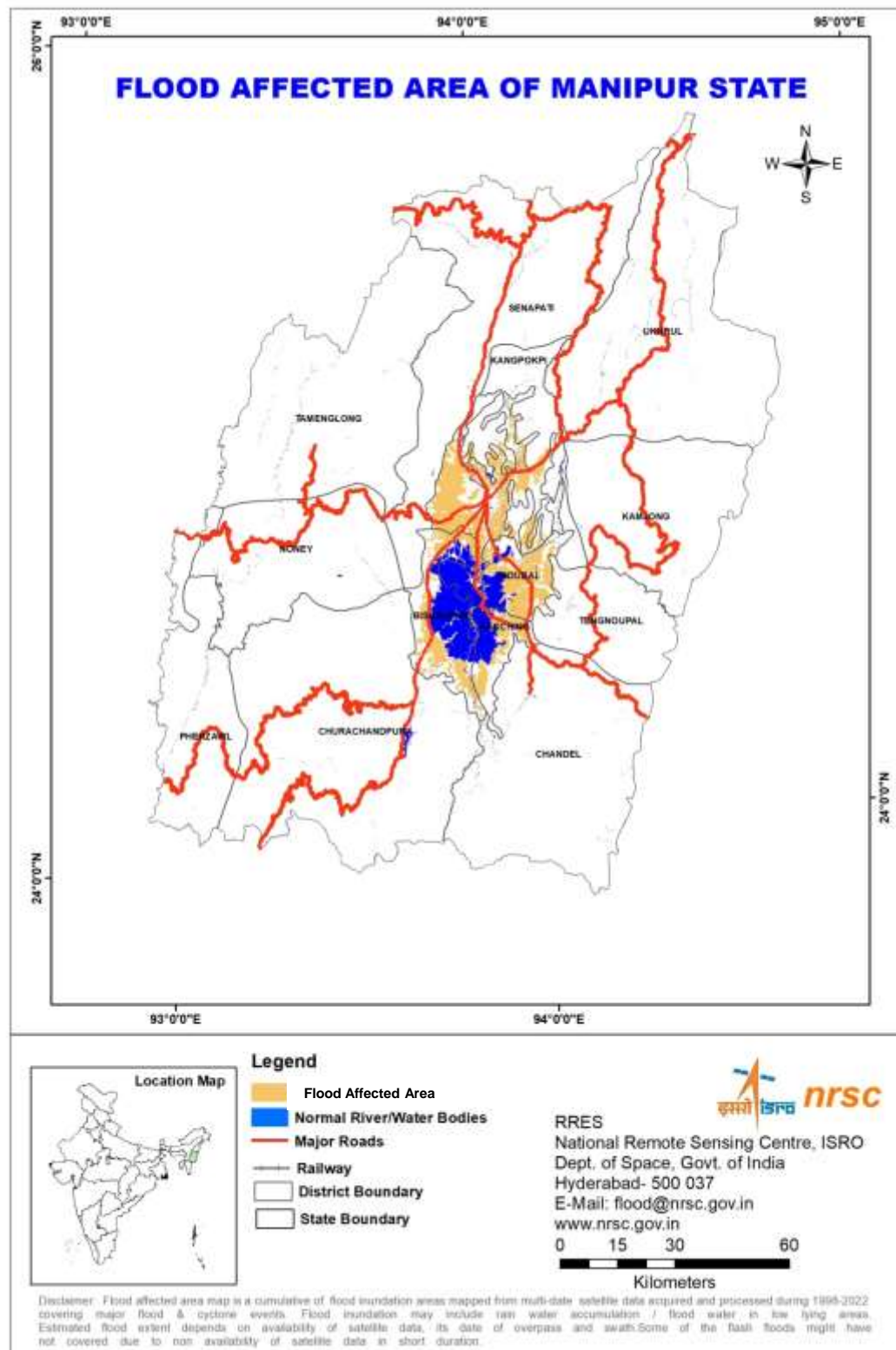
Fig.21.1. Flood affected area in Manipur State
